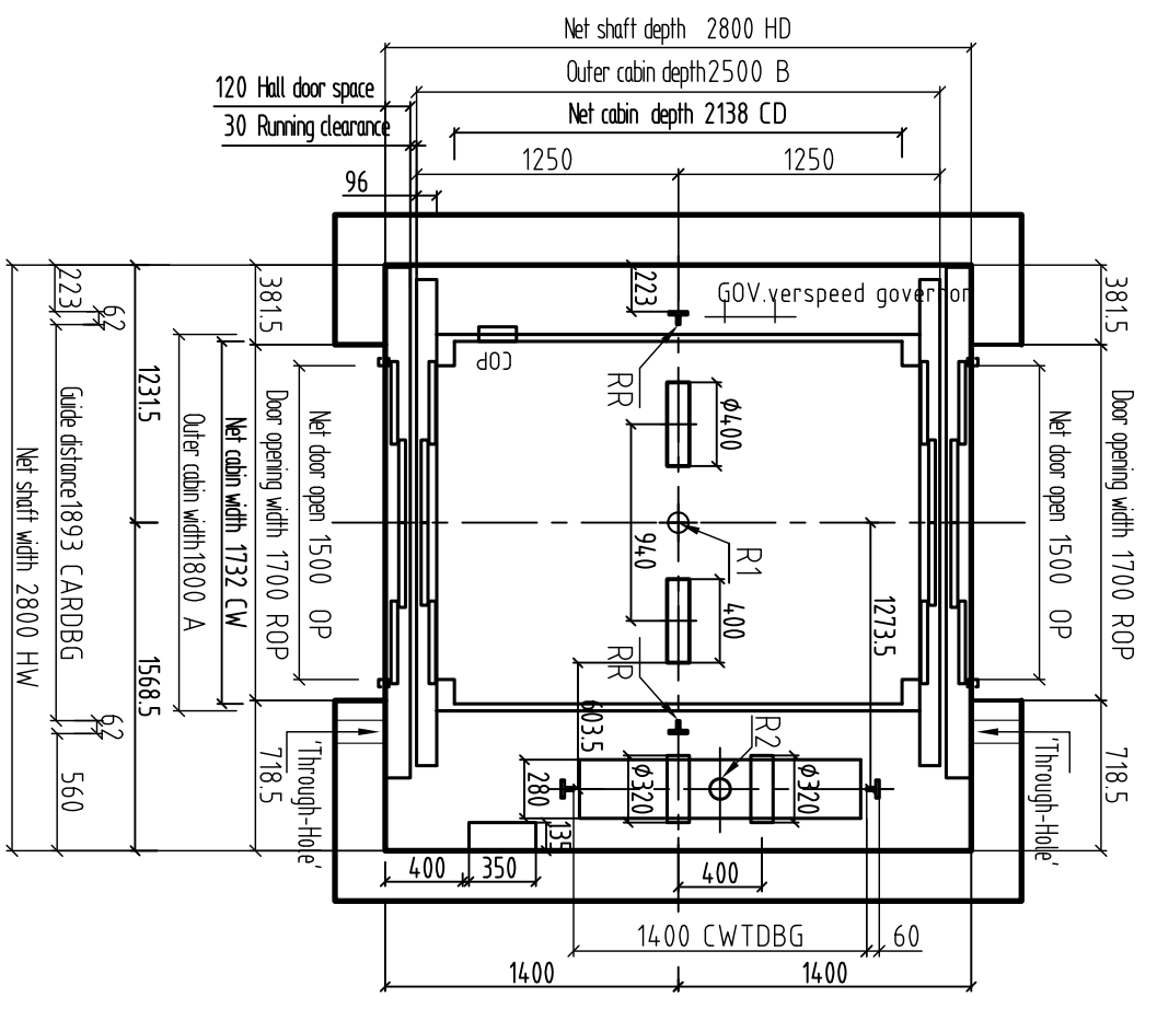
Plane figure of shaft
