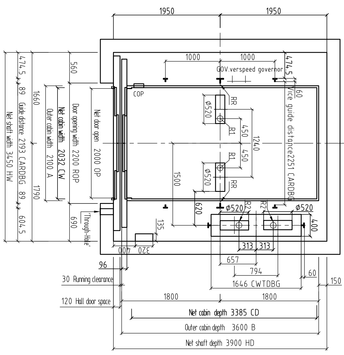
Plane figure of shaft
